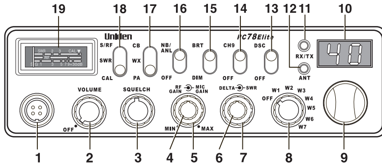
FRONT VIEW - PC78 Elite BACKLIGHTED PANEL
