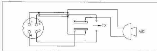
Fig. 1 Microphone Schematic
