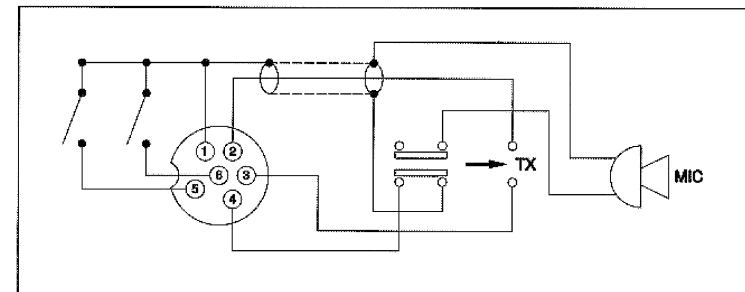
Transceiver Microphone Schematic Diagram
